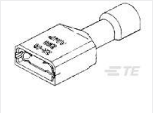
TE Part #3-350820-2 ULTRAFAST 250 ASSY REC 16-14 TPBR LP
