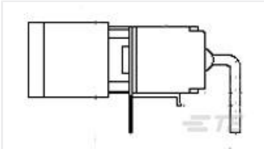
TE Part #1571986-8 A101J1AQ004=SGL POLE,ROCKER
