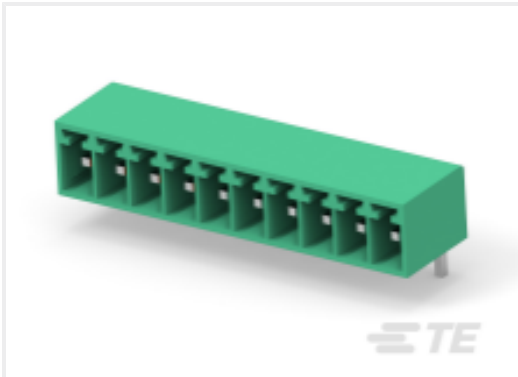
TE Part #1-2350514-0 10POS TB HDR 90 DEG, PITCH 3.5 &TL 3.5mm
