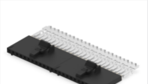
TE Part # 6-103957-1 2X12 MTE RCPT SR LATCH .100CL
