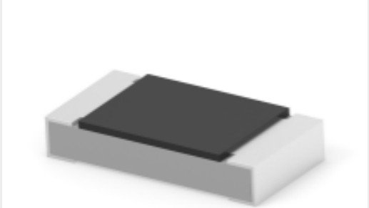
TE Part #2-2176581-5 RLC73PH 2B R10 1% 5K RL
