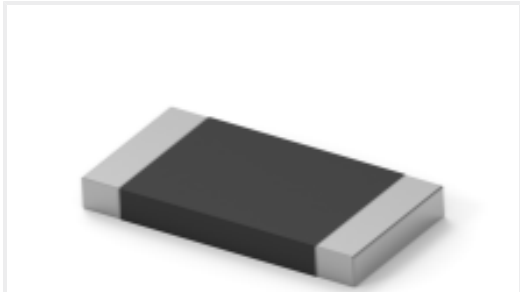
TE Part #8-2176421-9 TLRP 2512 2.0W R068 1% 75PPM 4K RL
