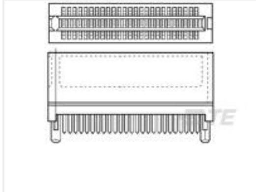
TE Part #5650719-1 STANDARD EDGE .050 SERIES 25 DUAL ASSY
