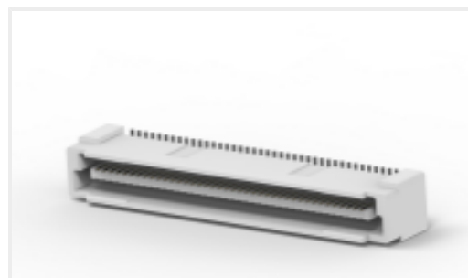
TE Part # CAT-313-PCB80 Free Height Plug Connector: Board-Board, Vertical, 80, 0.8mm
