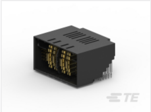
TE Part #2204440-1 MULTI-BEAM HD R/A PLUG 15S+2P+2P+15S
