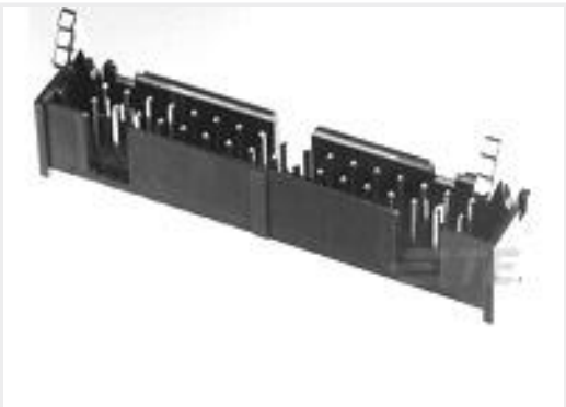
TE Part #1761608-7 IDC LOW PRO HDR 20P VERT SHT L
