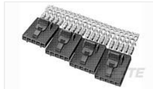
TE Part # 5-103958-6 2X7 MTE RCPT SR LATCH .100CL
