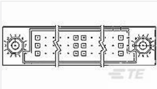
TE Part #532433-7 HDI PIN ASSY 3 ROW 150 POS
