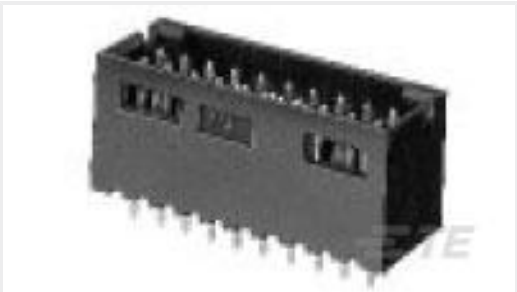
TE Part #1-102618-3 30 MODII HDR DRST SHRD .100CL
