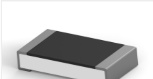
TE Part #9-2176388-7 RQ 1206 100R 0.1% 10PPM 5K RL
