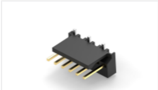
TE Part #CAT-104MTA-NVSMH PCB Header: Nylon, Vertical, Surface Mount, MTA 100
