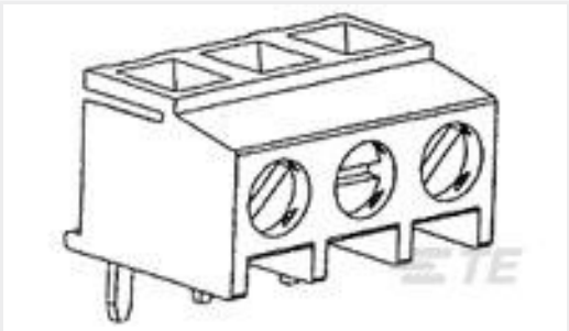
TE Part #284094-4 TERMI-BLOK PCB MOUNT 90, 5,08M
