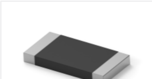
TE Part #4-2176422-8 TLRP 2512 3.0W R004 1% 50PPM 4K RL
