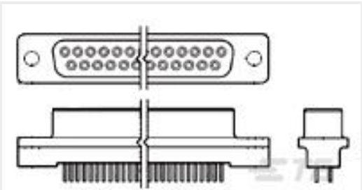
TE Part #5745058-3 HD-20 RCPT 25P VERT THD INS
