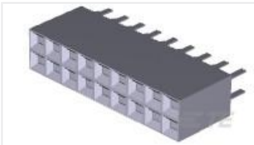
TE Part #5-534206-9 18 MODII VRT DR CE 100/115
