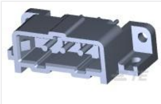
TE Part #207365-8 METRIMATE PIN HDR ASY,3P LF
