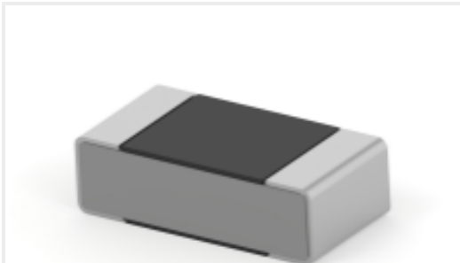
TE Part #1-2176280-2 CPF 0402 133K 0.1% 25PPM 1K RL
