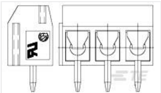
TE Part #1776244-4 4P TB ,90deg, VT, 5mm, Blue,w /interlock
