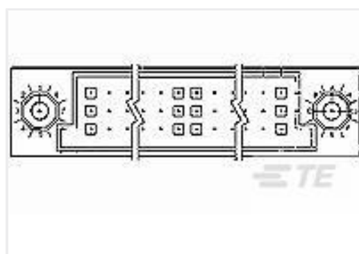
TE Part #532433-7 HDI PIN ASSY 3 ROW 150 POS
