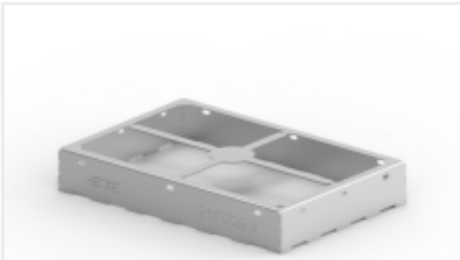
TE Part #2118722-2 STD SHIELD FRAME, CRS-38.10X25.40X6.00MM
