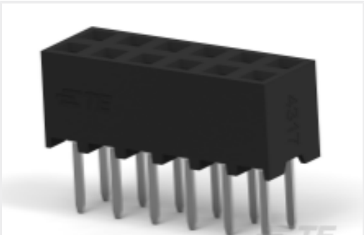
TE Part #1-2314820-4 14P,2MM,B-B,REC,DRVVT,2.7,0.1AU,TB
