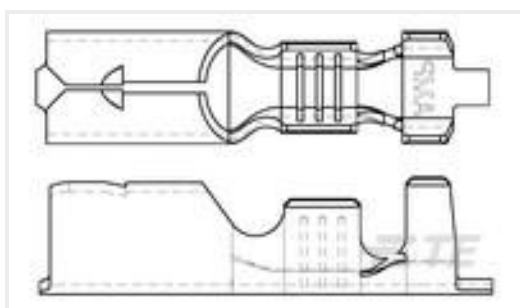
TE Part #881725-1 .156 DIA. SHUR PWG
