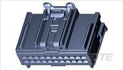
TE Part #3-1419158-0 INLIN CONN.FEMAL22P
