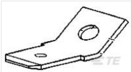
TE Part #60465-1 250 FASTON TAB BR
