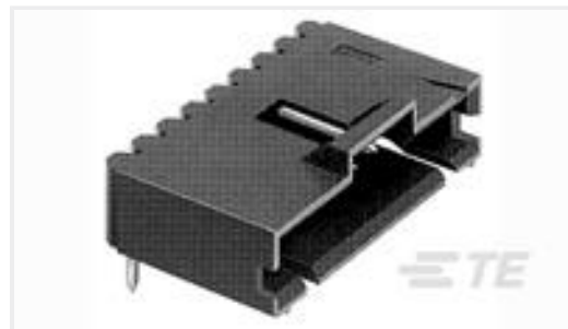
TE Part #5-104935-2 08 MTE HDR SRR LATCH
