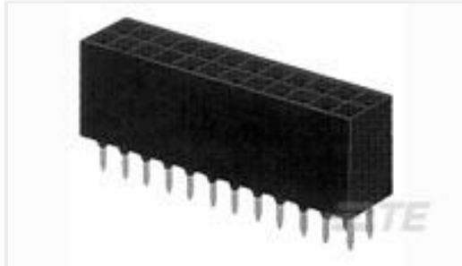
TE Part # 2-215307-1 2X21P HV100 REC CON. TE, 7.0MM
