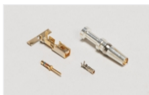
Connector Contacts(94)
