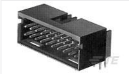
TE Part #6-103673-3 14 MTE HDR SRRA LATCH W/HLDWN
