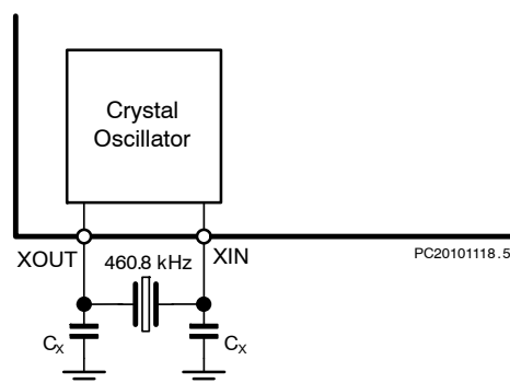
Figure 11. Crystal Oscillator
