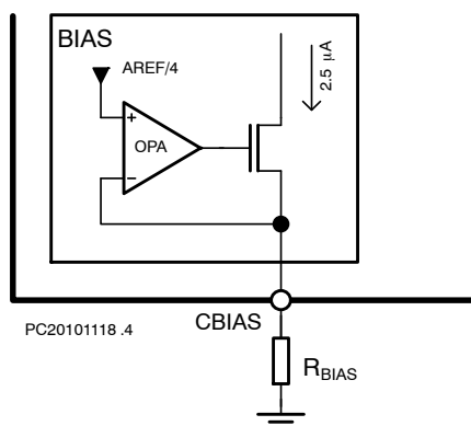
Figure 10. Bias Circuit
