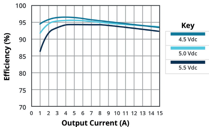
EFFICIENCY VS OUTPUT CURRENT VPOL15A-5-SIP ( V_o = 1.8 Vdc)
