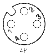
Pin Assignments Front View
