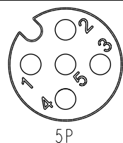
Pin Assignments Front View
