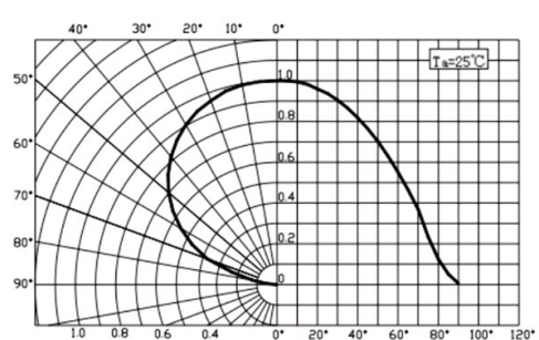
Radiation Diagram
