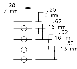
HOLE DETAIL
