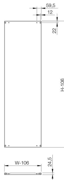
Mounting plate
