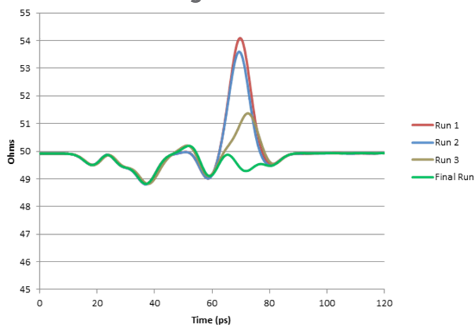
TDR Design Iterations
