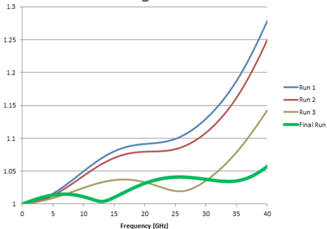
VSWR Design Iterations
