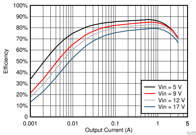
Figure 7-9. V_{OUT} = 0.95 V Efficiency, L = 1.2 \mu H
