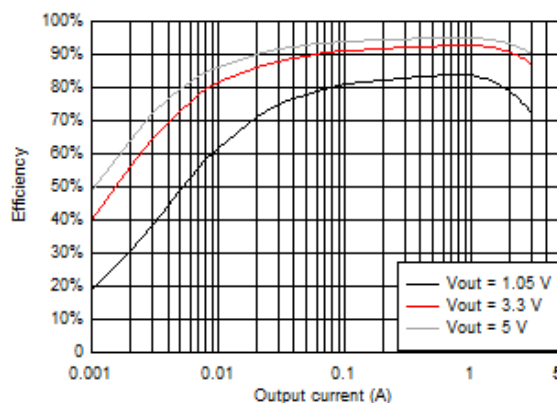
TPS563202S Efficiency
