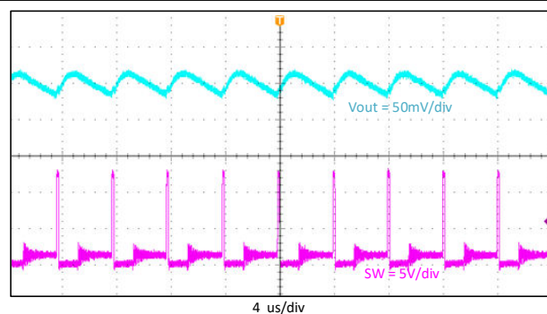
Figure 9-6. Output Voltage Ripple, I_{out} = 0.3\text{ A}
