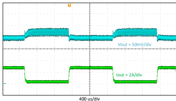
Figure 9-8. Transient Load Response, 0.3 to 2.7 A
