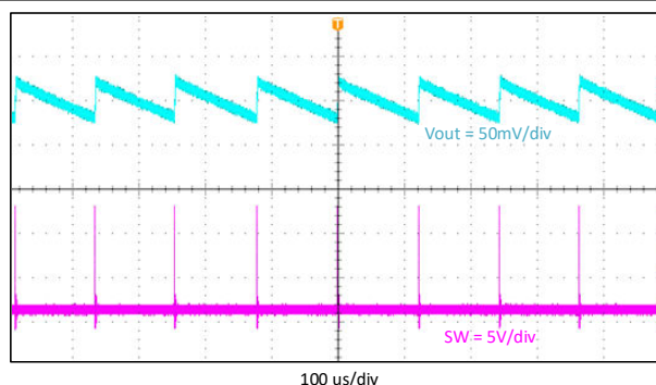
Figure 9-5. Output Voltage Ripple, 10 mA
