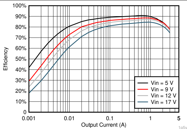
Figure 7-11. V_{OUT} = 1.5 V Efficiency, L = 1.5 \mu H
