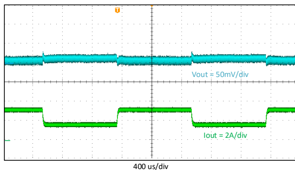
Figure 9-9. Transient Load Response, 1.5 to 3 A
