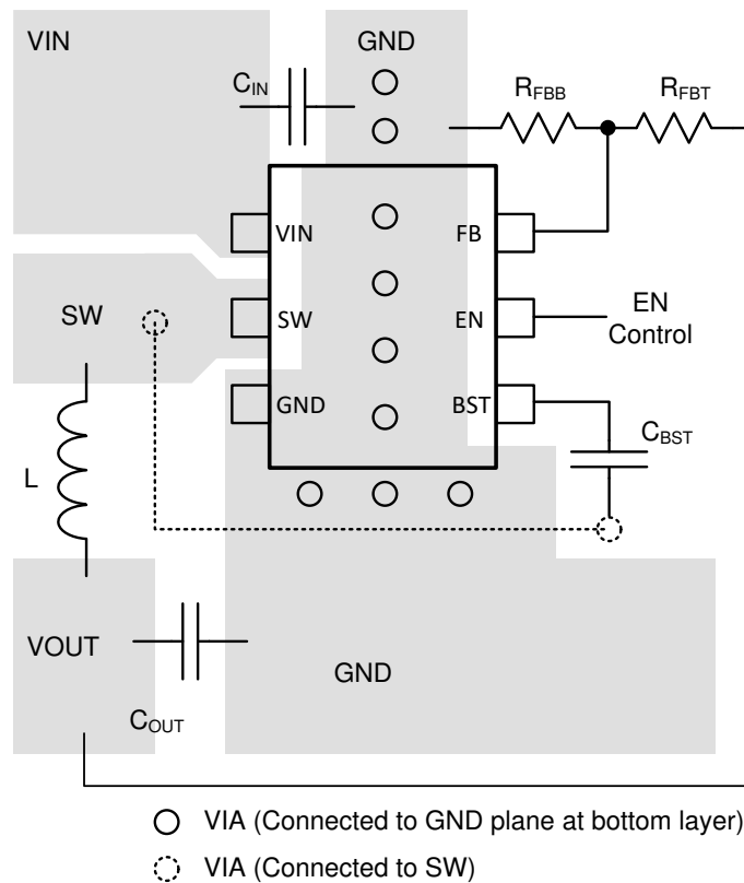
Figure 11-1. TPS563202S Layout
