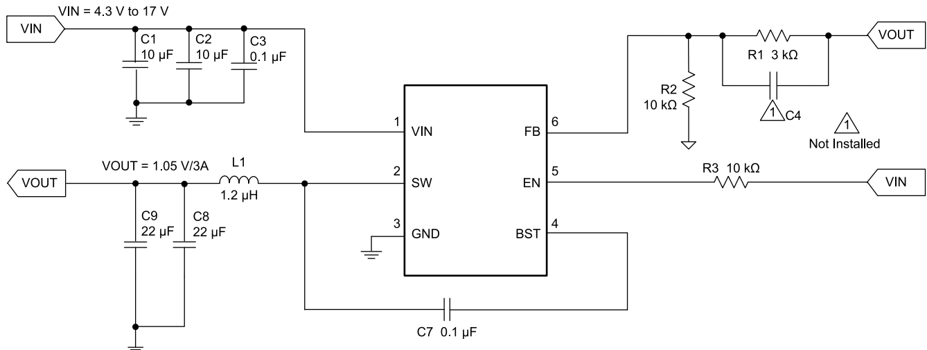
Figure 9-1. TPS563202S 1.05-V/3-A Reference Design
