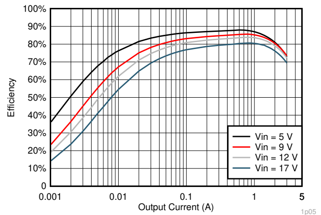
Figure 7-10. V_{OUT} = 1.05 V Efficiency, L = 1.2 \mu H
