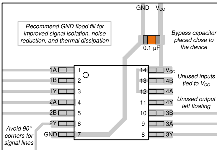
Figure 9-3. Example Layout for the SNx4AHC86
