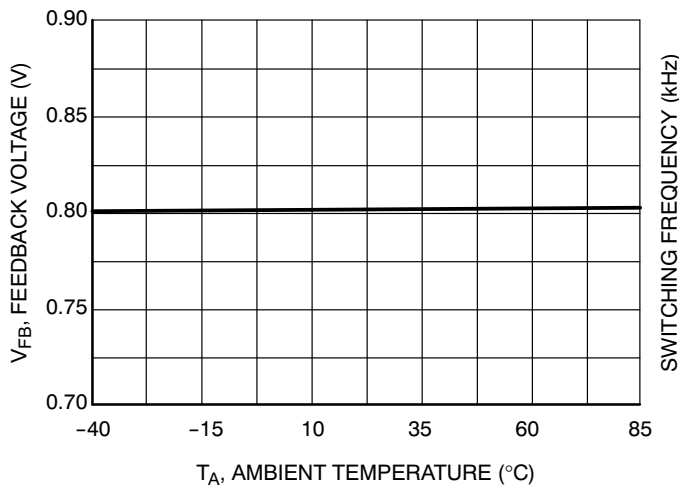
Figure 6. V_{FB} Feed Back Voltage vs. Ambient Temperature
