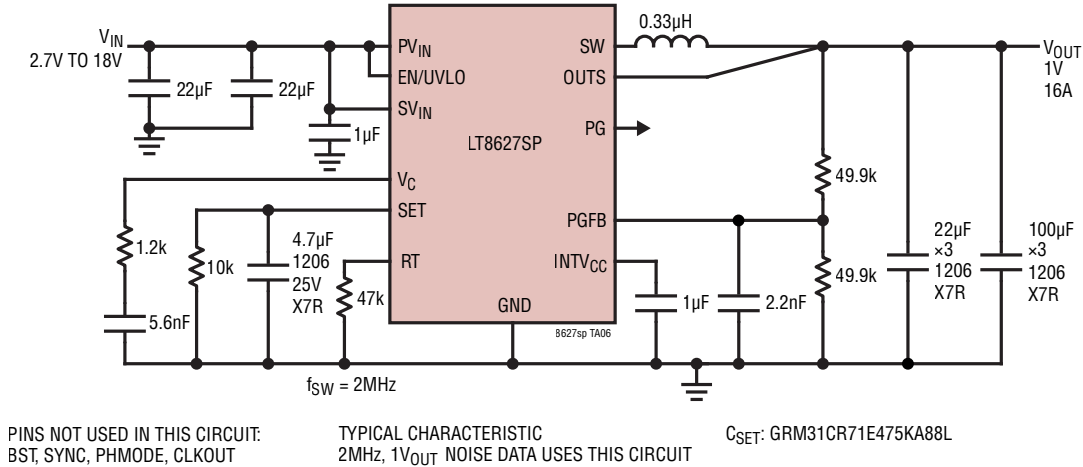
1V 16A 2MHz Step-Down Converter with Soft-Start, Fast Start-up and Power Good
