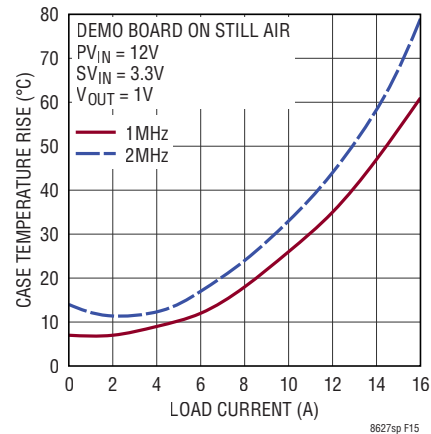
Figure 15. Case Temperature Rise
