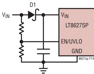
Figure 14. Reverse V_{IN} Protection
