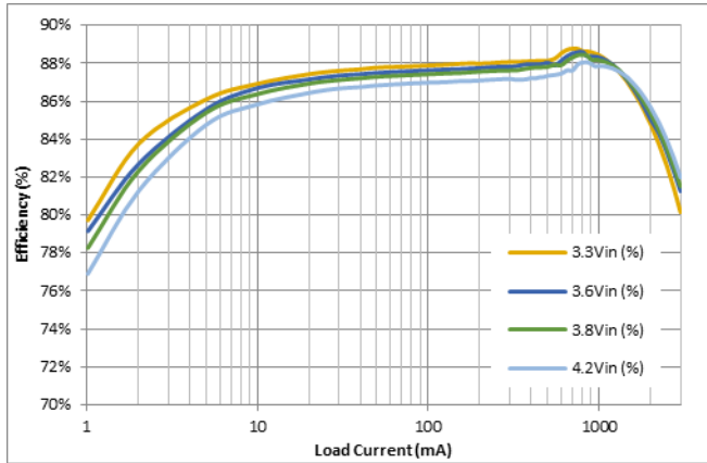
Figure 5. Efficiency vs. Load Current and Input Voltage, V_{OUT}=1.15625\text{ V}
