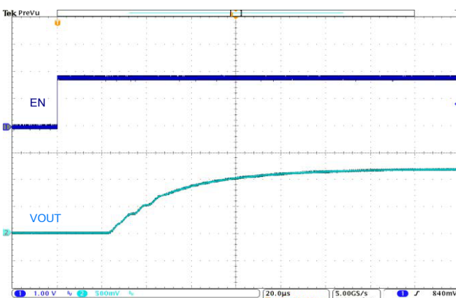
Figure 15. Startup, 5 \Omega Load, V_{OUT} = 1.15625\text{ V} , V_{IN} = 3.6\text{ V}
