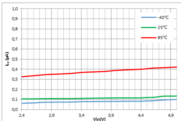
Figure 12. Shutdown Current vs. Input Voltage and Temperature
