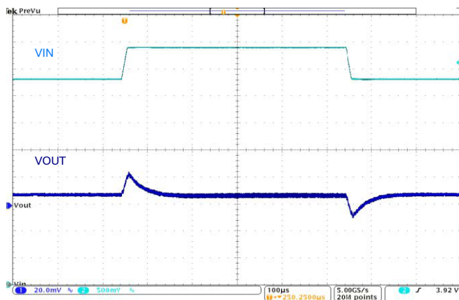
Figure 13. Line Transient, 3.6–4.2 V_{IN} , 1.15625 V_{OUT} , 10 \mu\text{s} Edge at 1 A Load
