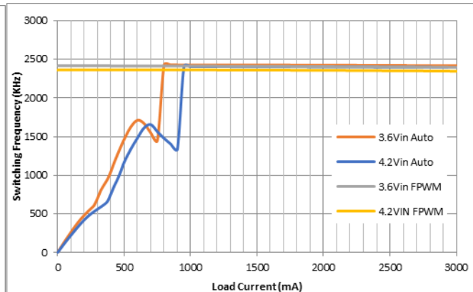
Figure 10. Frequency vs. Load Current, V_{IN}=4.2\text{ V} and 3.6\text{ V} , V_{OUT}=1.15625\text{ V} , Auto PWM
